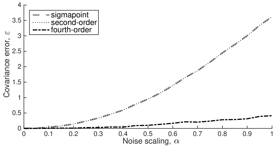
Figure 7.7 Results from Compound Experiment: error, \varepsilon , in computing covariance associated with compounding two poses using three methods, as compared to Monte Carlo. The sigmapoint and second-order methods are algebraically equivalent for this problem and thus appear the same on the plot. The input covariances were gradually scaled up via the parameter, \alpha , highlighting the improved performance of the fourth-order method.
